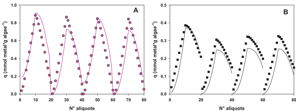
Fig. 8. Adsorption/desorption of (A) Cd ( C_0 = 1 \text{ mM} ) and (B) Pb ( C_0 = 0.5 \text{ mM} ) by U. lactuca fixed in columns at pH 5.5. The symbols correspond to experimental results, while solid lines were calculated using Eqs. (2) and (3), the experimental values of inner and outer concentrations and the flux of mobile phases.
