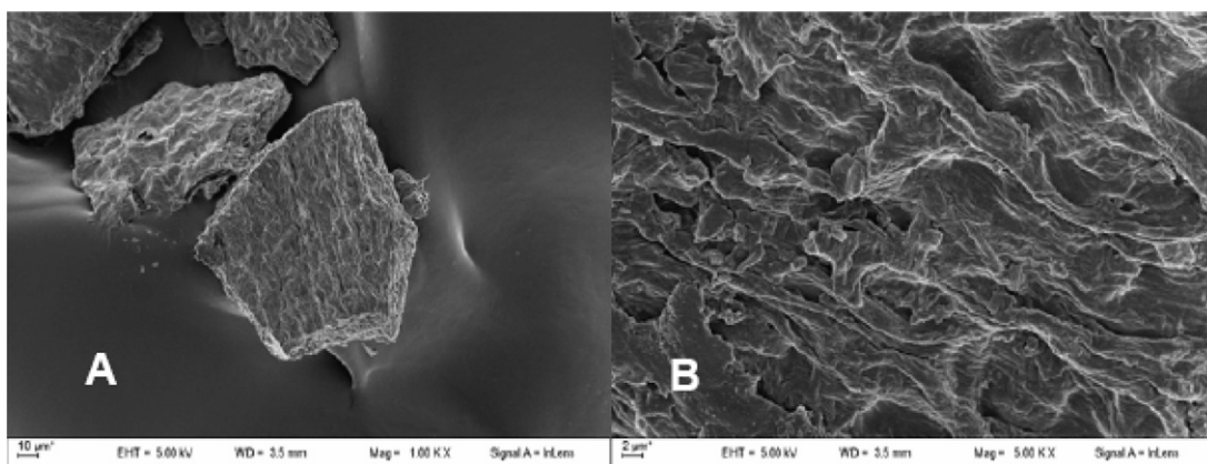
Fig. 5. U. lactuca SEM images at two magnifications (A: 1000× and B: 5000×) and 5 kV.
