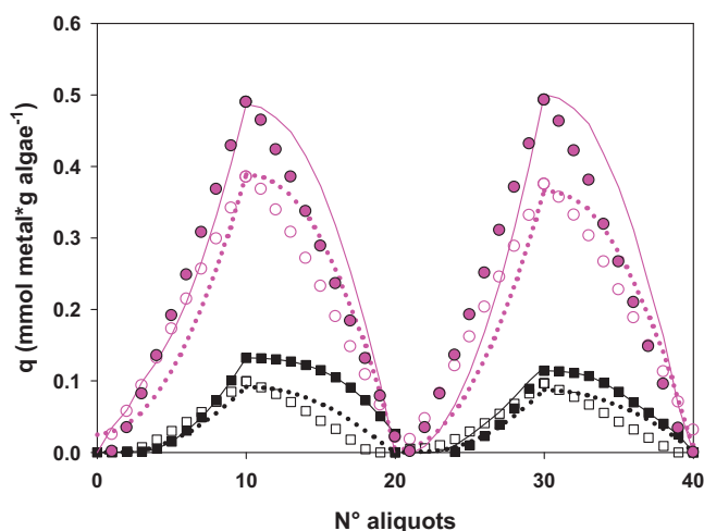
Fig. 9. Cd ( \circ ) adsorption/desorption in the presence of Pb and Pb ( \square ) adsorption/desorption in the presence of Cd at pH 5.5 by U. lactuca packed in columns compared to the adsorption/desorption process of Cd ( \bullet ) and Pb ( \blacksquare ) when there is no contribution of any other ion in solution. The symbols correspond to experimental results, while lines were calculated using Eqs. (2) and (3), the experimental values of inner and outer concentrations and the flux of mobile phases.
